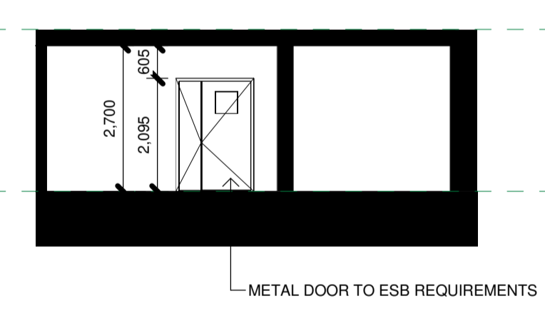
Substation Block H Section 1 : 100
