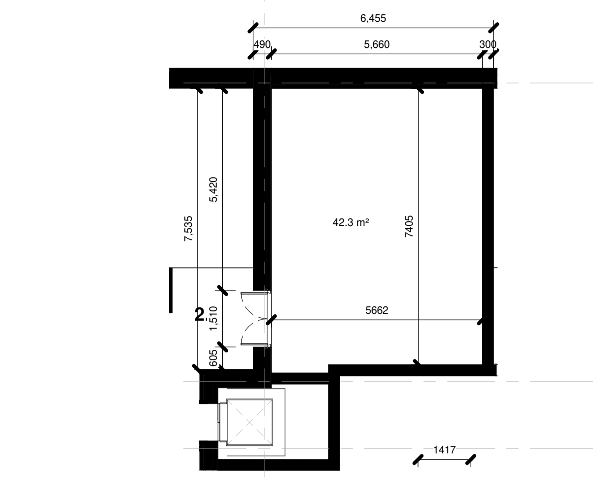
Refuse Block A Plan Copy 1 1 : 100
